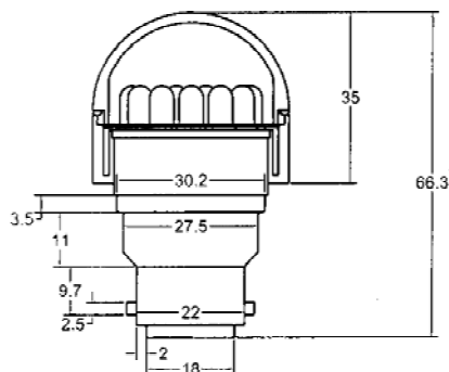
B22 Bayonet Cap
